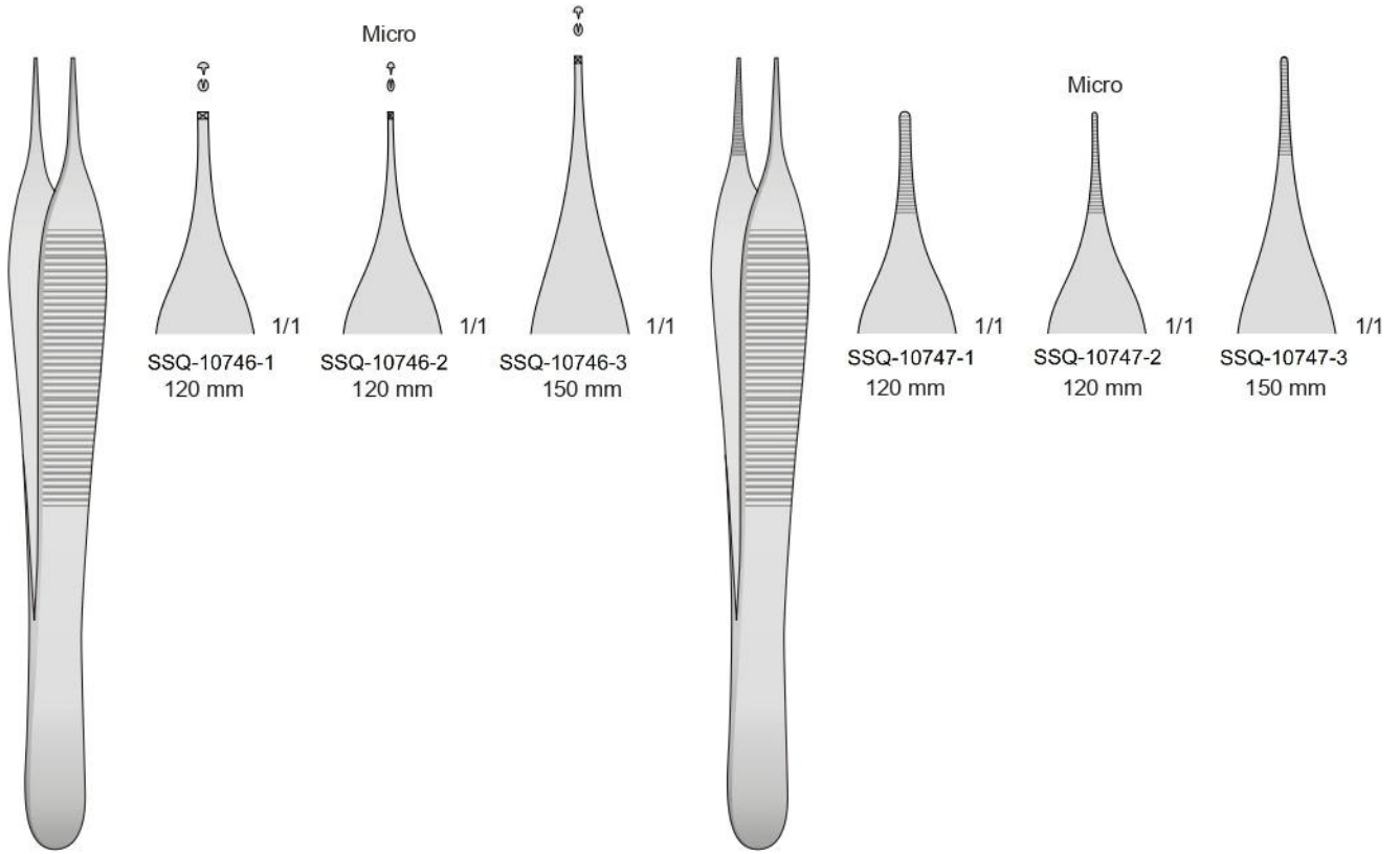
ADSON SSQ-10746
